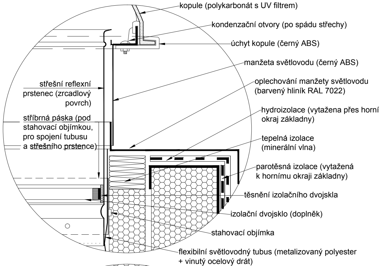
detail B
